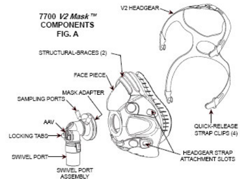
Oro-Nasal BiLevel V2 Mask™ with Headgear
